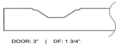
VC-MD 3050 Raised Panel
